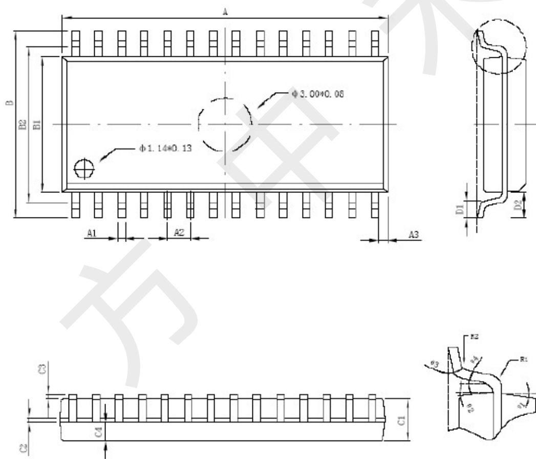
DETAIL "X"
